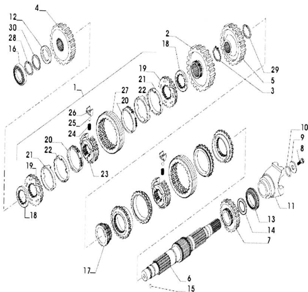
в. Secondary shaft
